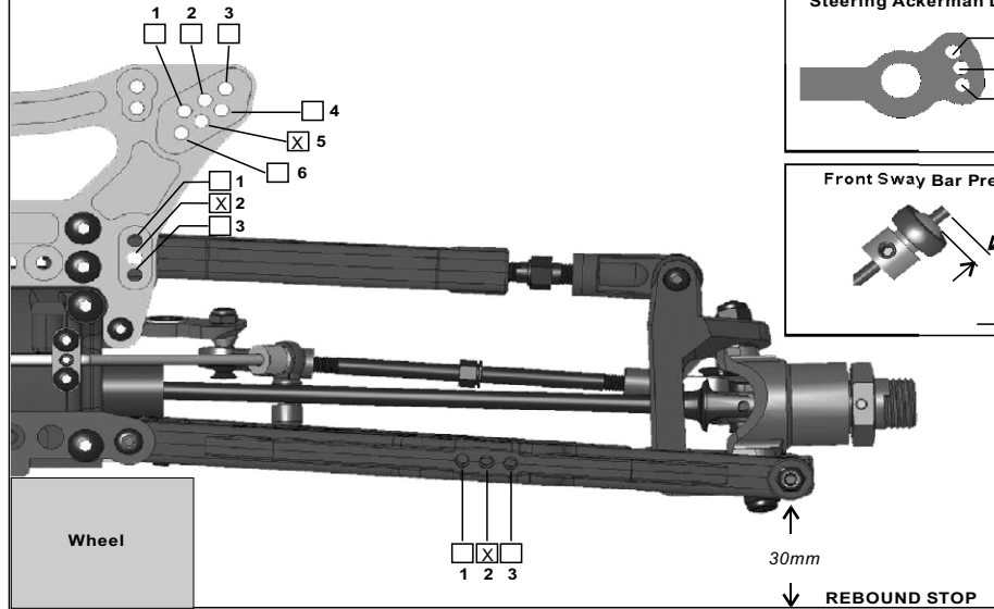
Steering Ackerman Location
